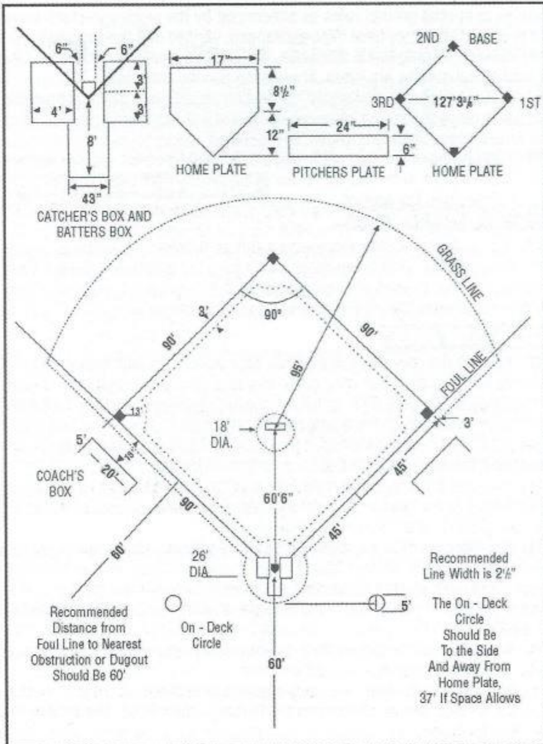
Diagram 2 Official Measurements . . . for laying out baseball field
