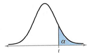
Right-tailed test
