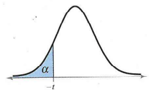
Left-tailed test
