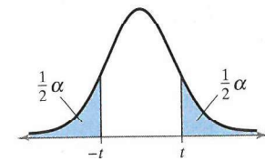
Two-tailed test
